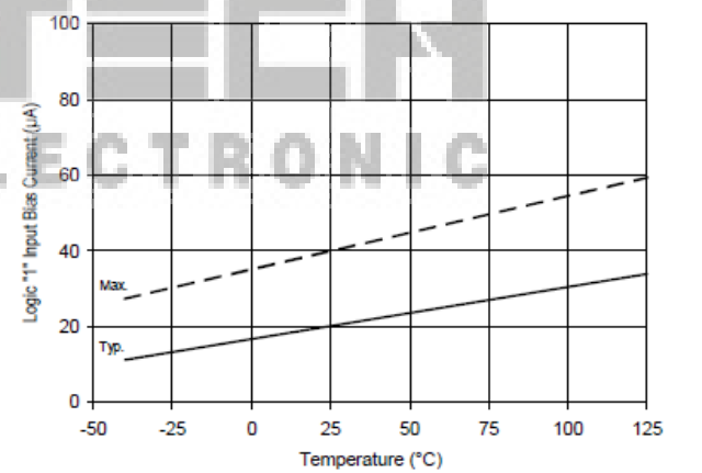
Figure 18A. Logic '1' Input Current vs. Temperature
